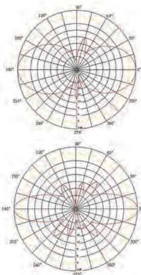
Horizontal Pattern (698-960/1710-2170)
